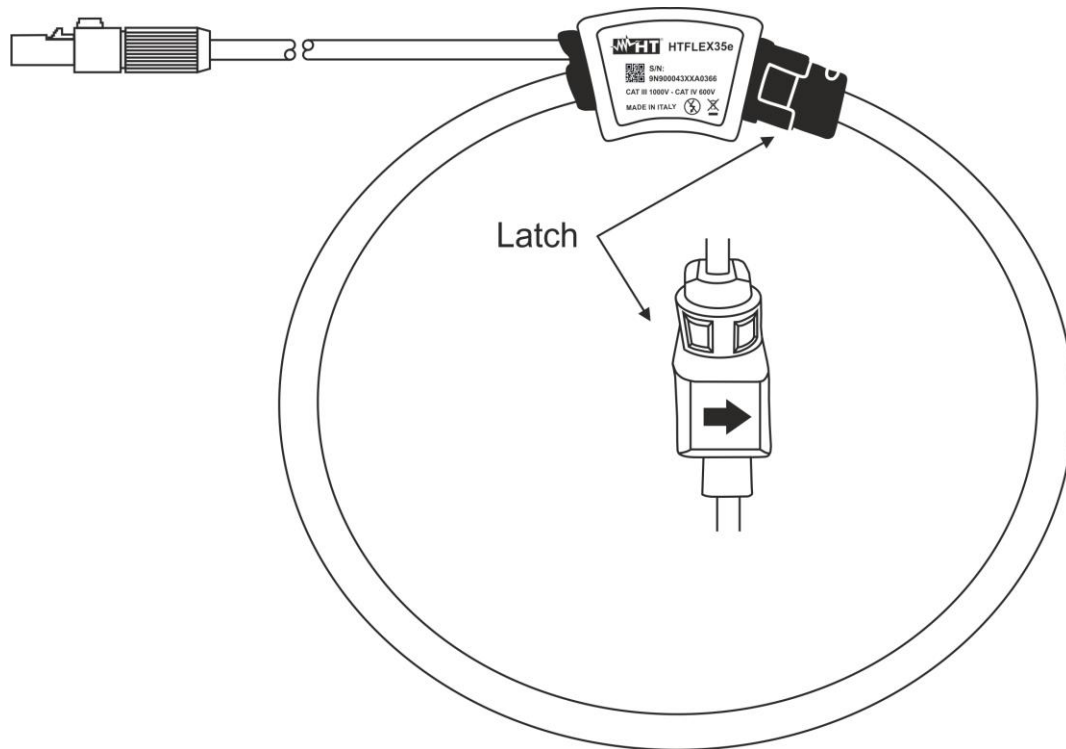
Fig. 2: HTFLEX35e transducer description
