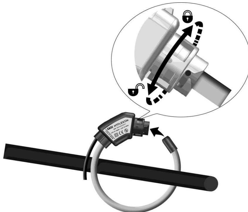
Fig. 3: Connection of HTFLEX33e clamp on a conductor
