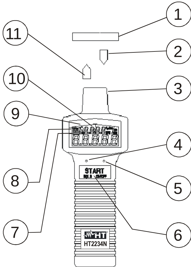
Fig. 1: panelo frontal
