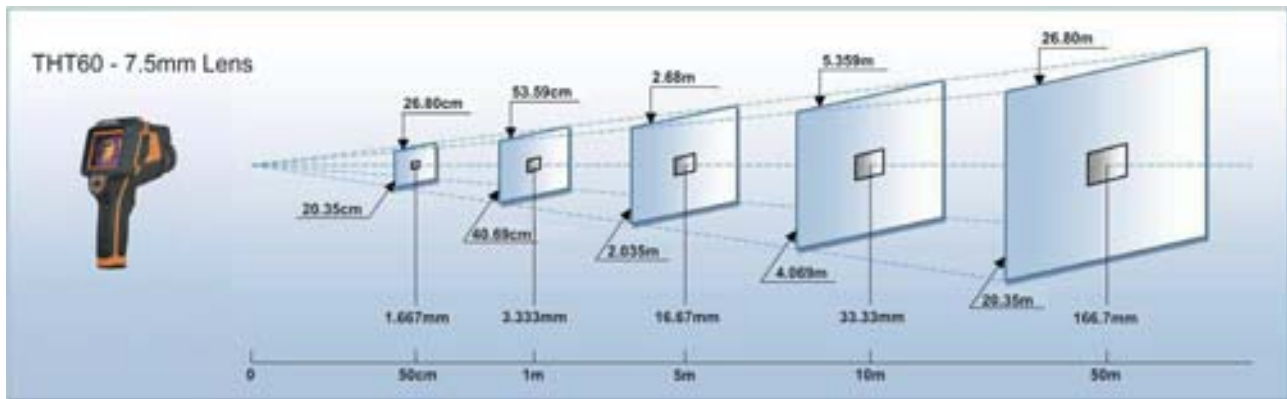
Fig. 72: Representation of the instruments D/S ratio (THT60)
