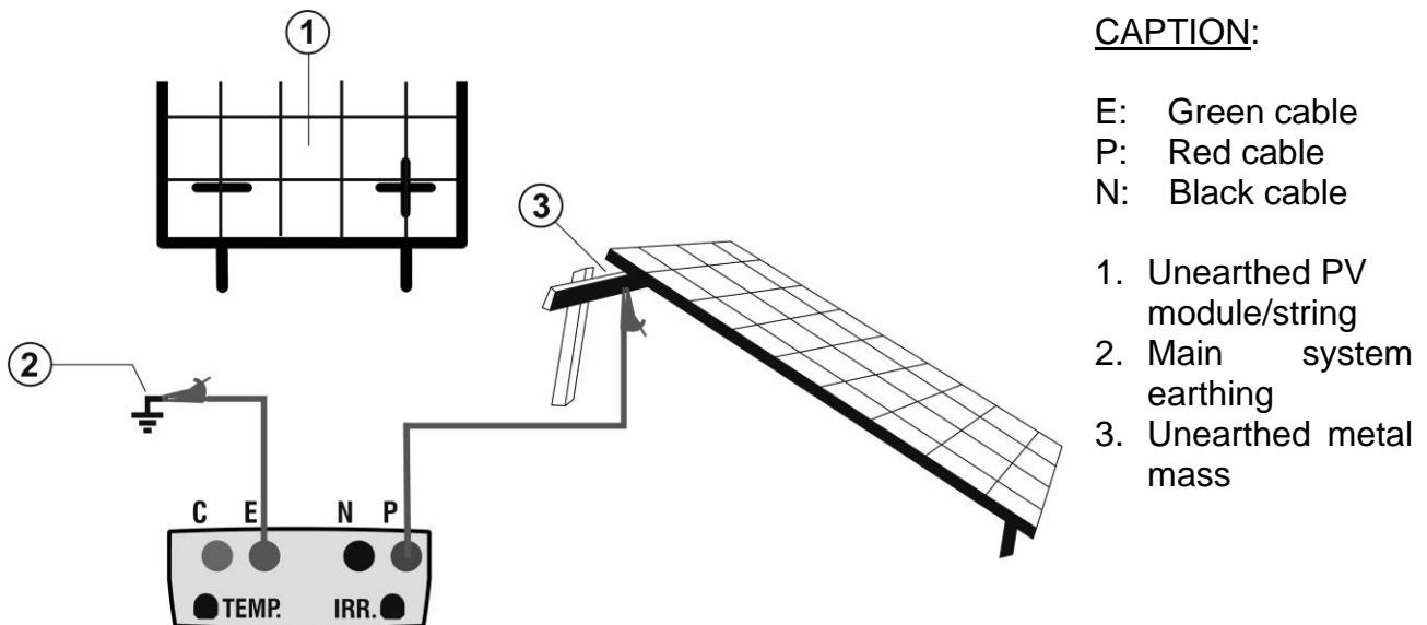
Fig. 11: Instrument connection for insulation measurement in TIMER mode
