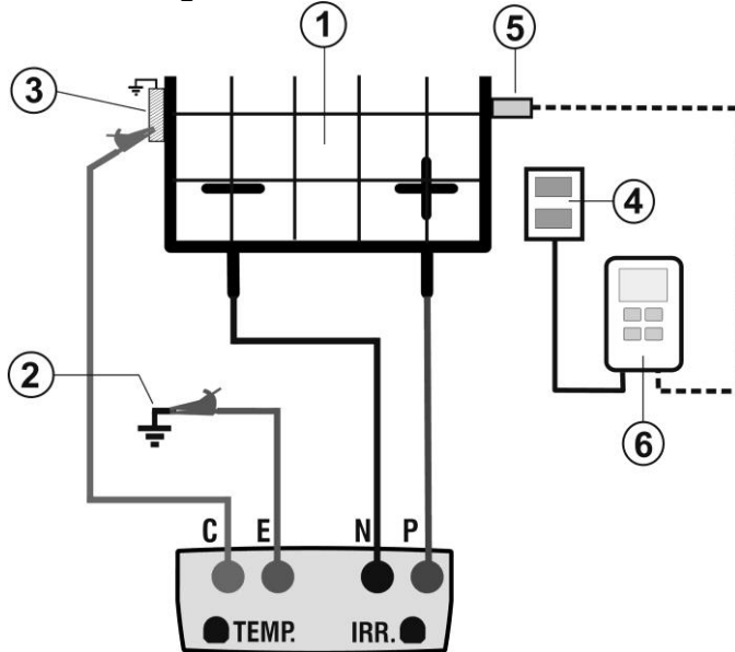
Fig. 8: Connection for IVCK test with direct irradiance measurement
