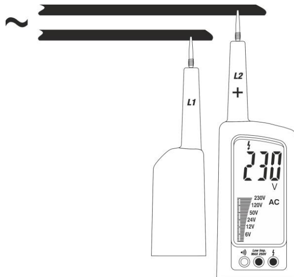
Fig. 4: AC Voltage measurement with low input impedance
