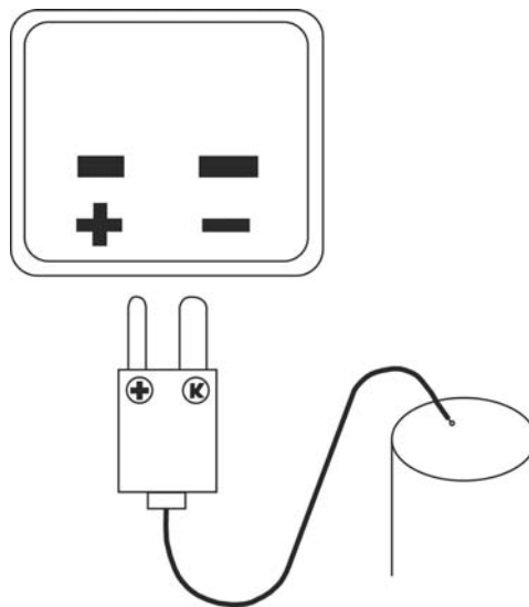
Fig. 5: Connection of K-type probe in the instrument
